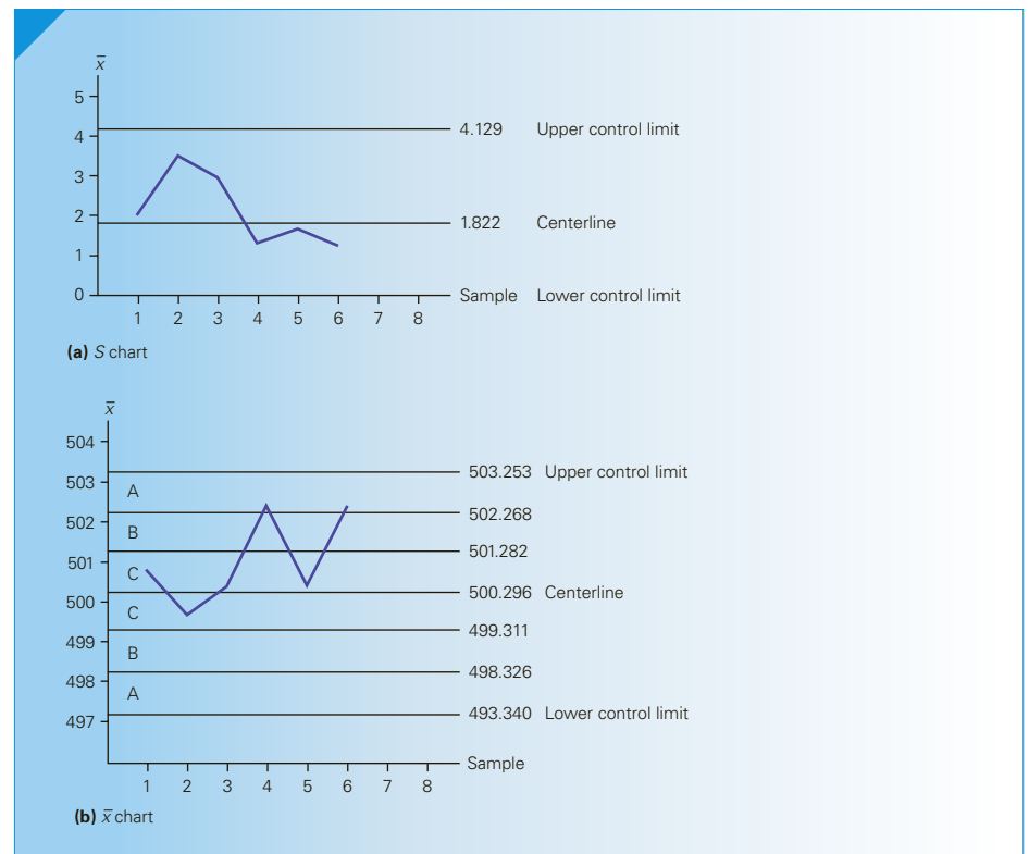
FIGURE 21.9 S and \bar{x} Charts for Example 21.3
