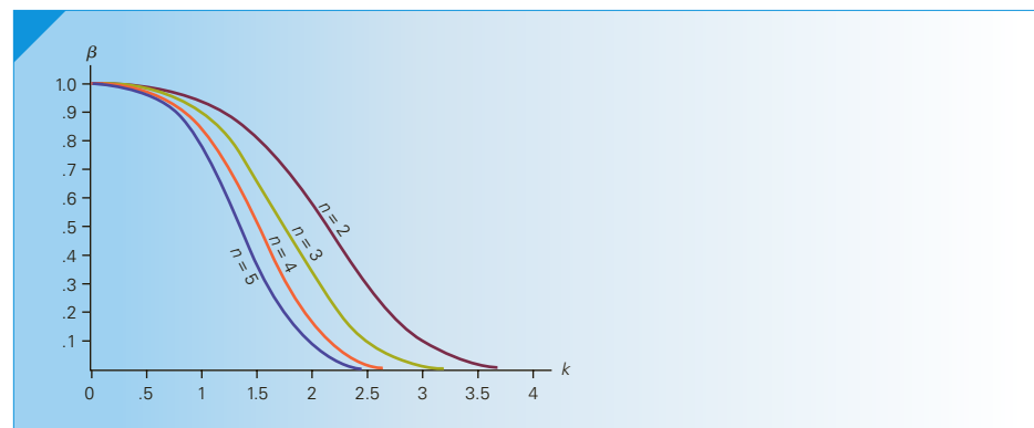
FIGURE 21.3 Operating Characteristic Curve for n = 2, 3, 4, and 5
