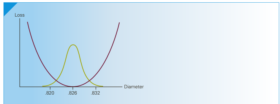
FIGURE 14.9 Taguchi Loss Function and the Distribution of Piston Rings
