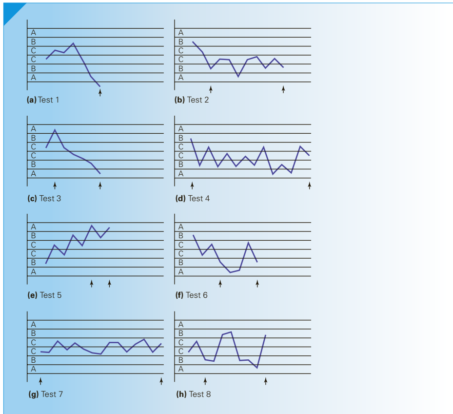
FIGURE 21.7 Examples of Patterns Indicating Process Out of Control
