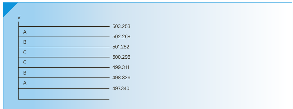
FIGURE 21.6 Zones of \bar{x} Chart: Example 21.1
