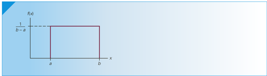
FIGURE 8.4 Uniform Distribution
