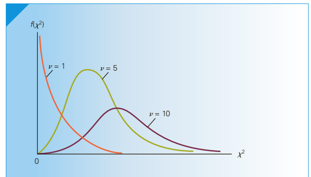
FIGURE 8.28 Chi-Squared Distribution with \nu = 1, 5, and 10
