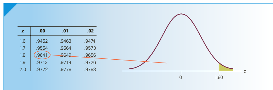
FIGURE 8.13 P(Z > 1.80)
