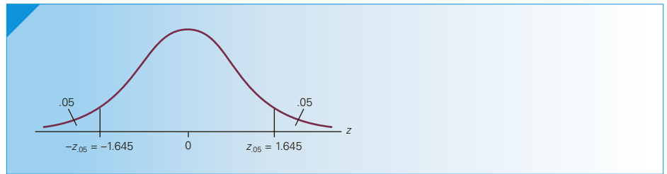
FIGURE 8.18 -Z_{.05}
