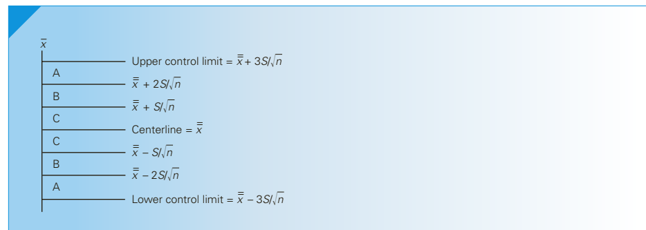
FIGURE 21.5 Zones of \bar{x} Chart
