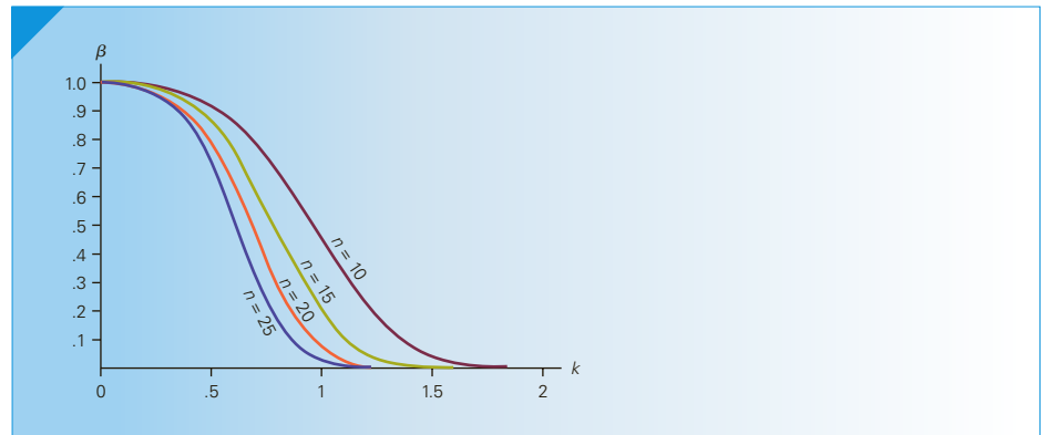
FIGURE 21.4 Operating Characteristic Curve for n = 10, 15, 20, and 25
