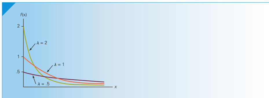
FIGURE 8.21 Exponential Distributions
