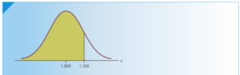
FIGURE 8.10 P(X < 1,100)
