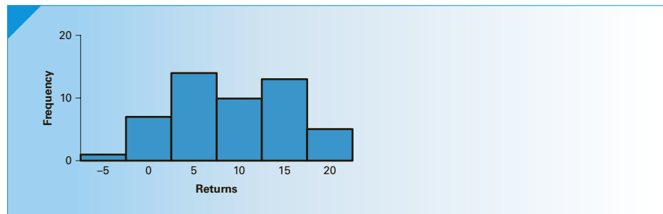
FIGURE 13.2 Histogram of Rates of Return for Directly Purchased Mutual Funds in Example 13.1
