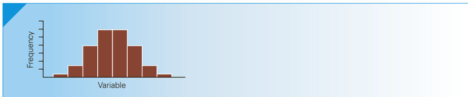
FIGURE 3.6 Bell-Shaped Histogram
