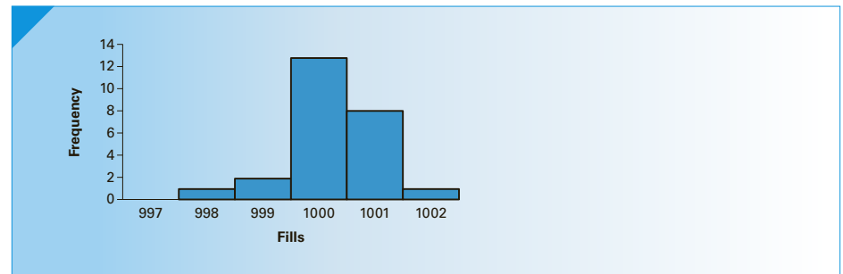
FIGURE 12.5 Histogram for Examples 12.3 and 12.4
