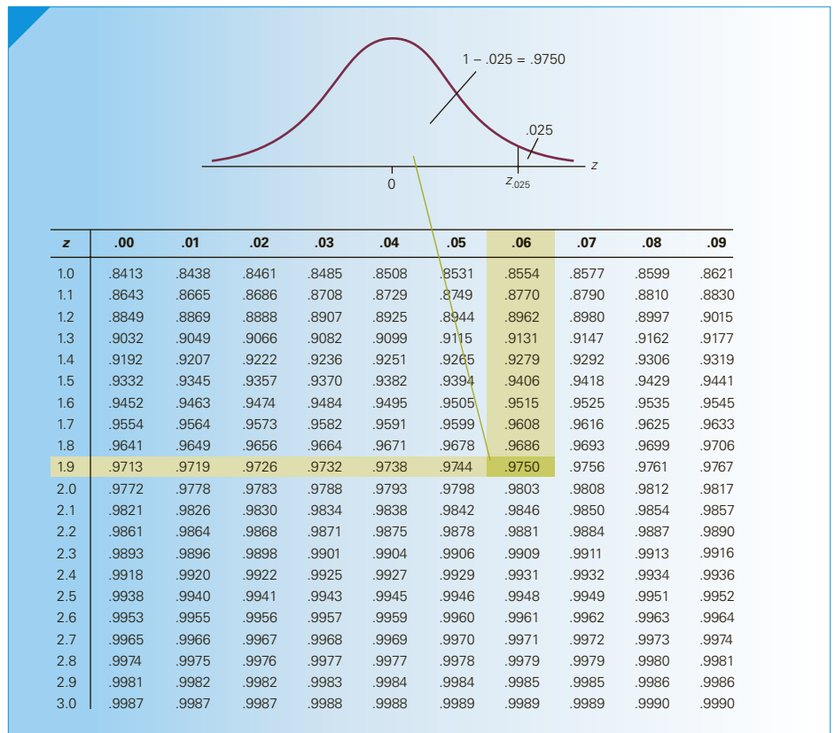
FIGURE 8.16 Z_{.025}
