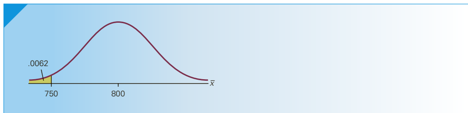
FIGURE 9.5 P(\bar{X} < 750)
