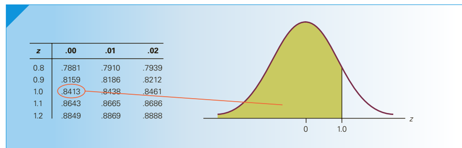
FIGURE 8.12 P(Z < 1.00)
