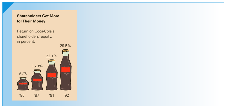
FIGURE 3.19 Correct Pictogram
