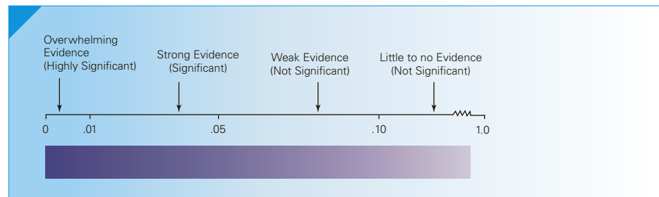
FIGURE 11.6 Describing p -Values
