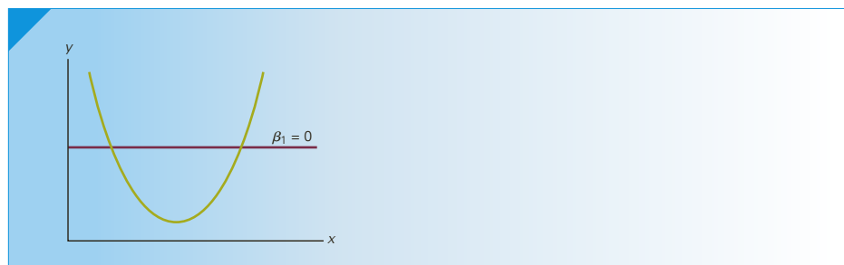
FIGURE 16.6 Quadratic Relationship
