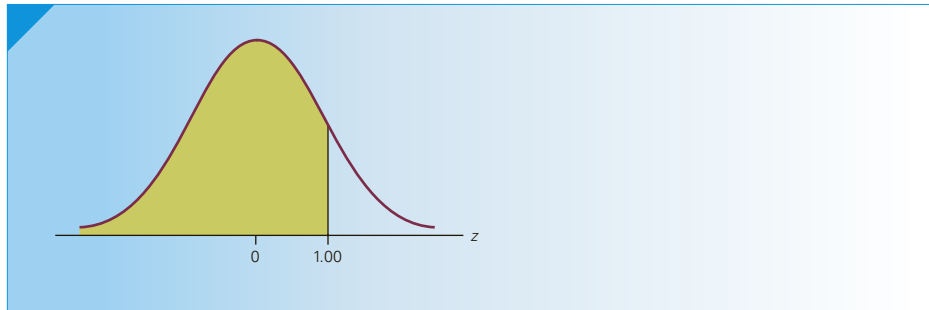
FIGURE 8.11 P(Z < 1.00)
