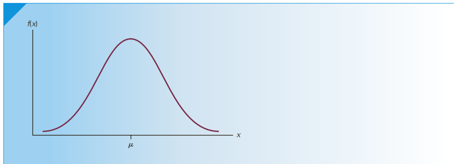
FIGURE 8.7 Normal Distribution
