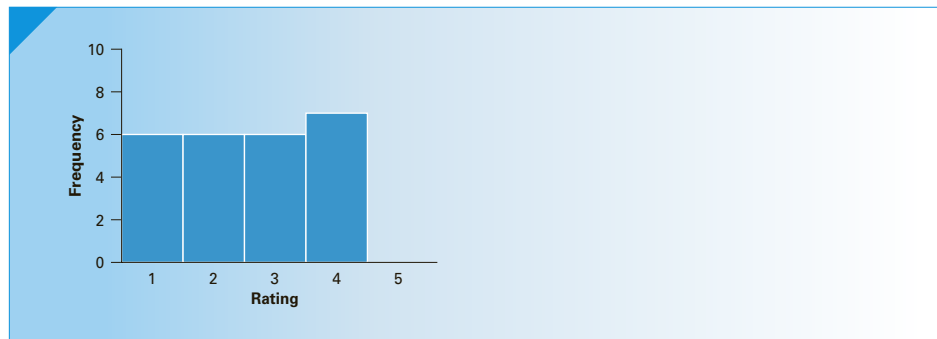
FIGURE 19.8 Histogram of Ratings of North American Car in Example 19.4
