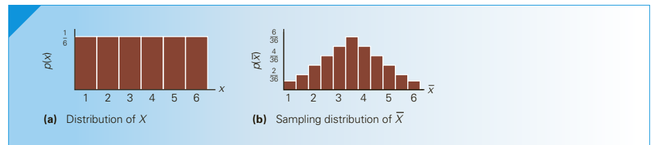
FIGURE 9.2 Distributions of X and \bar{X}
