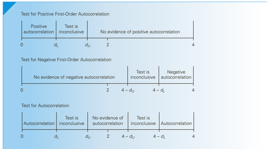
FIGURE 17.5 Durbin-Watson Test
