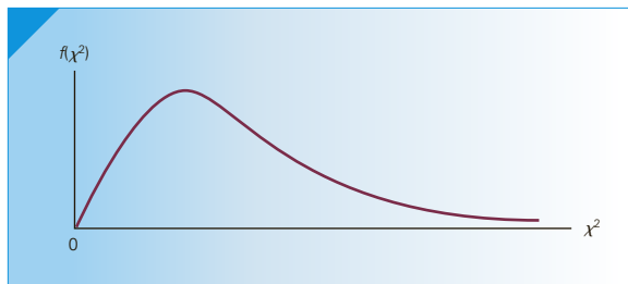
FIGURE 8.27 Chi-Squared Distribution
