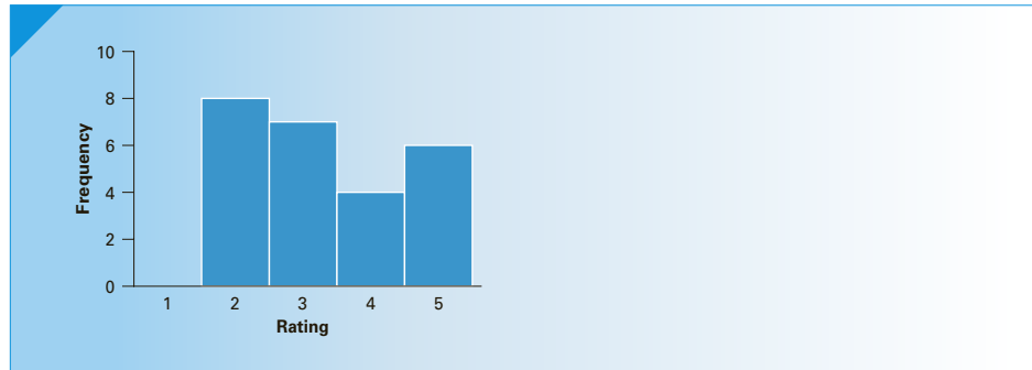
FIGURE 19.8 Histogram of Ratings of North American Car in Example 19.4
