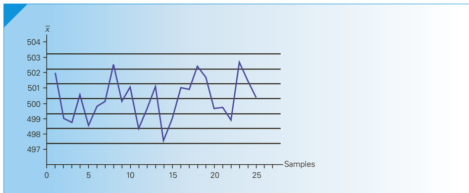
FIGURE 21.8 \bar{x} Chart with Zones: Example 21.1
