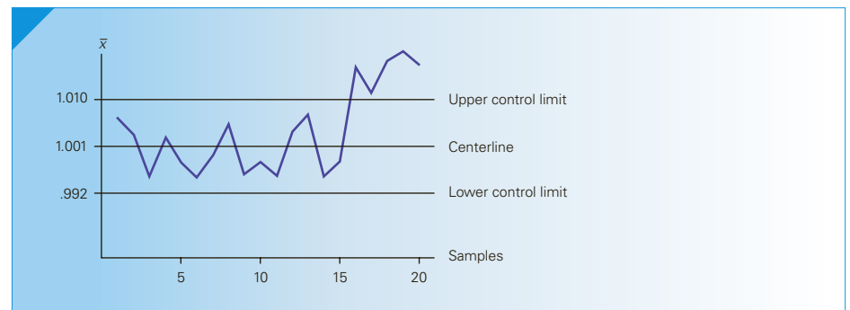
FIGURE 21.2 \bar{x} Chart: Process Out of Control
