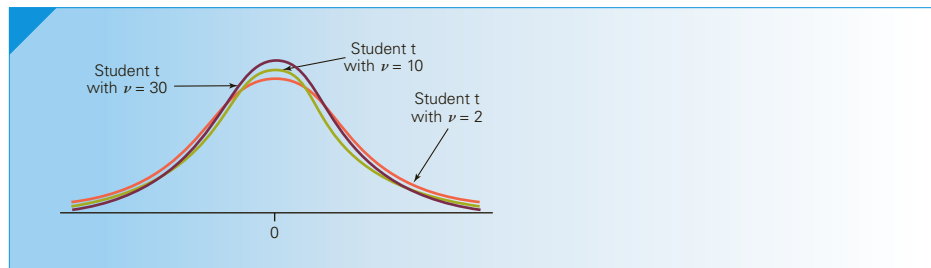
FIGURE 8.25 Student t Distribution with \nu = 2, 10 , and 30
