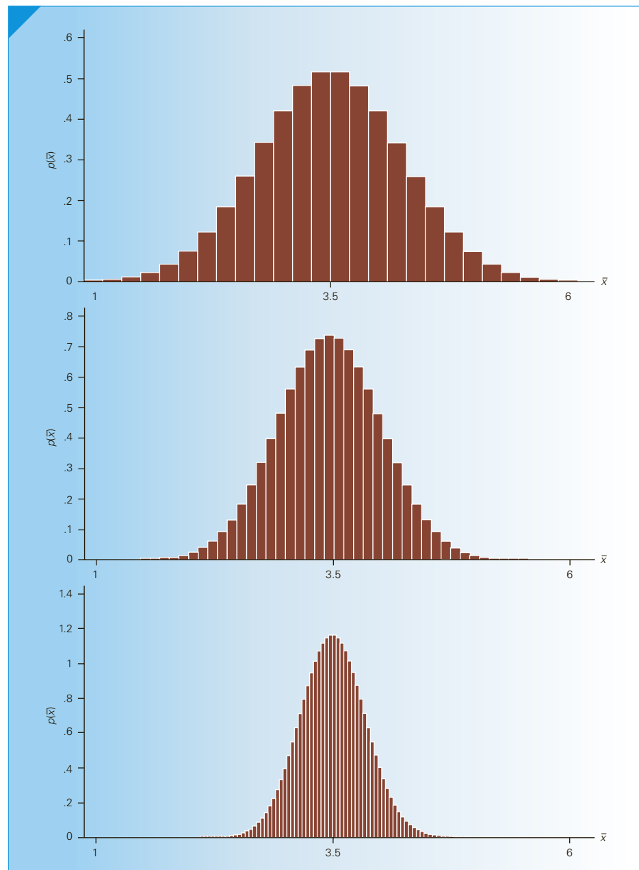
FIGURE 9.3 Sampling Distributions of \bar{X} for n = 5, 10 , and 25
