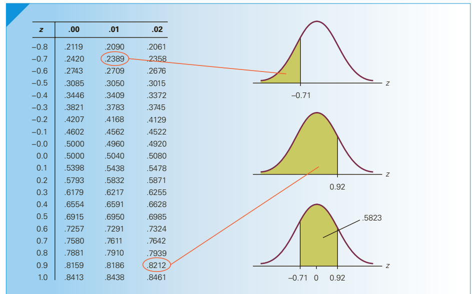
FIGURE 8.14 P(-0.71 < Z < 0.92)
