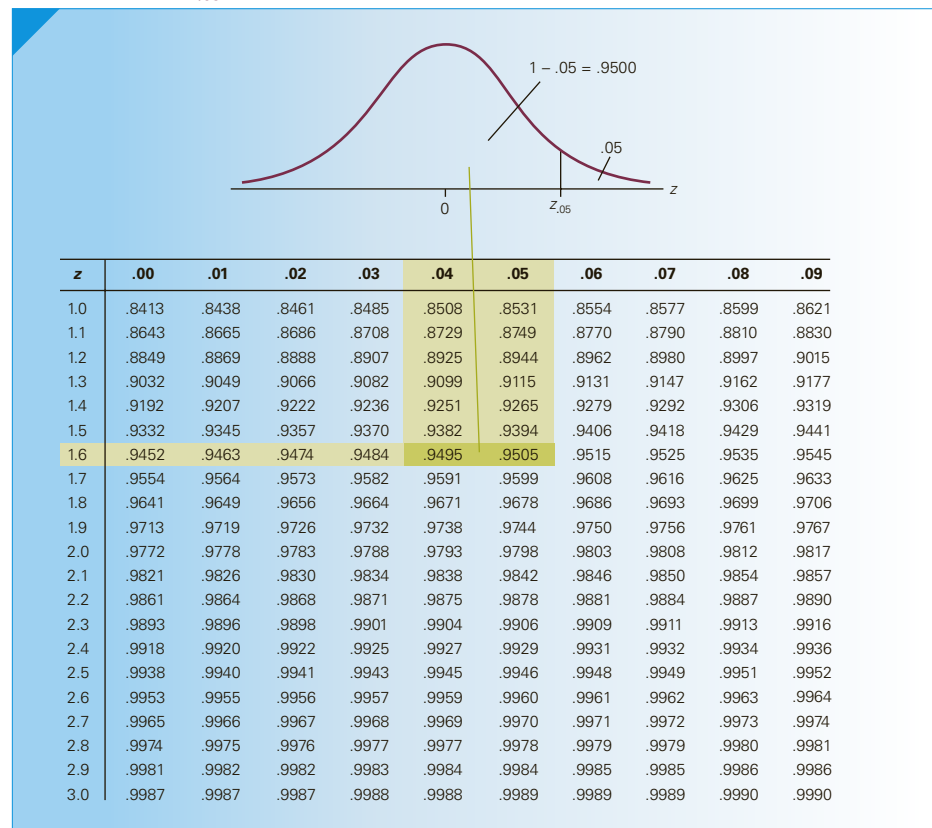
FIGURE 8.17 Z_{.05}
