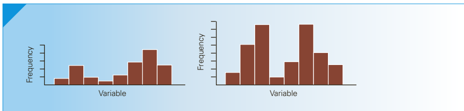
FIGURE 3.5 Bimodal Histograms
