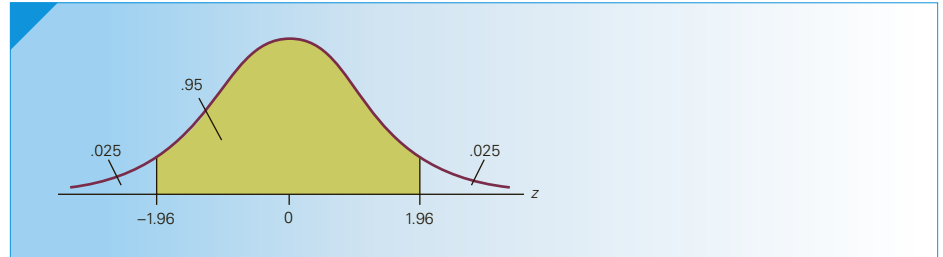
FIGURE 9.6 P(-1.96 < Z < 1.96) = .95
