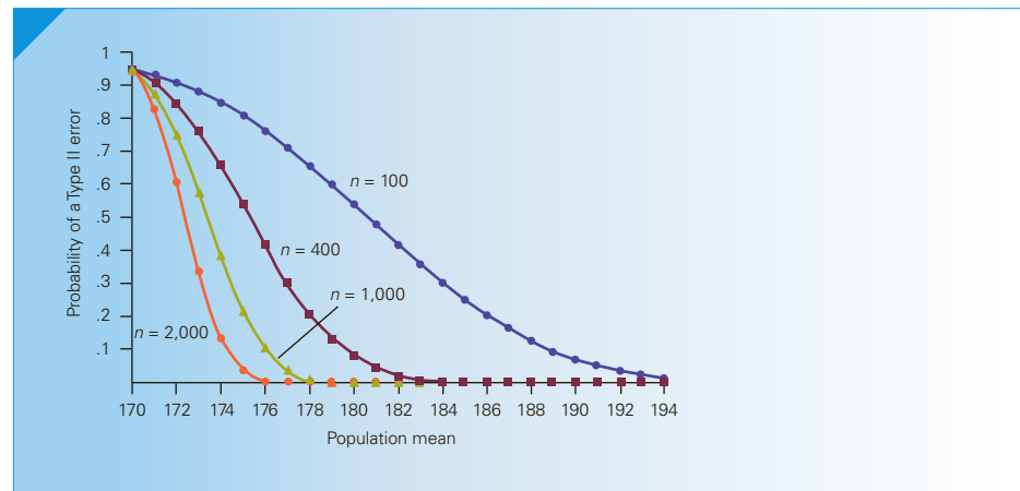
FIGURE 11.13 Operating Characteristic Curve for Example 11.1 for n = 100, 400, 1,000, and 2,000
