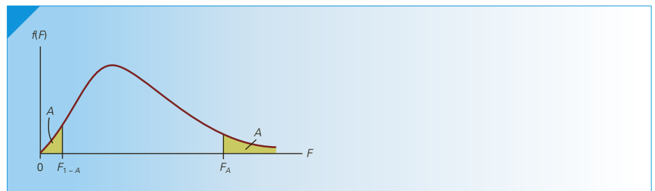
FIGURE 8.31 F_{1-A} and F_A
