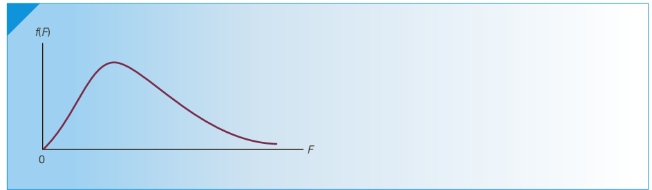
FIGURE 8.30 F Distribution
