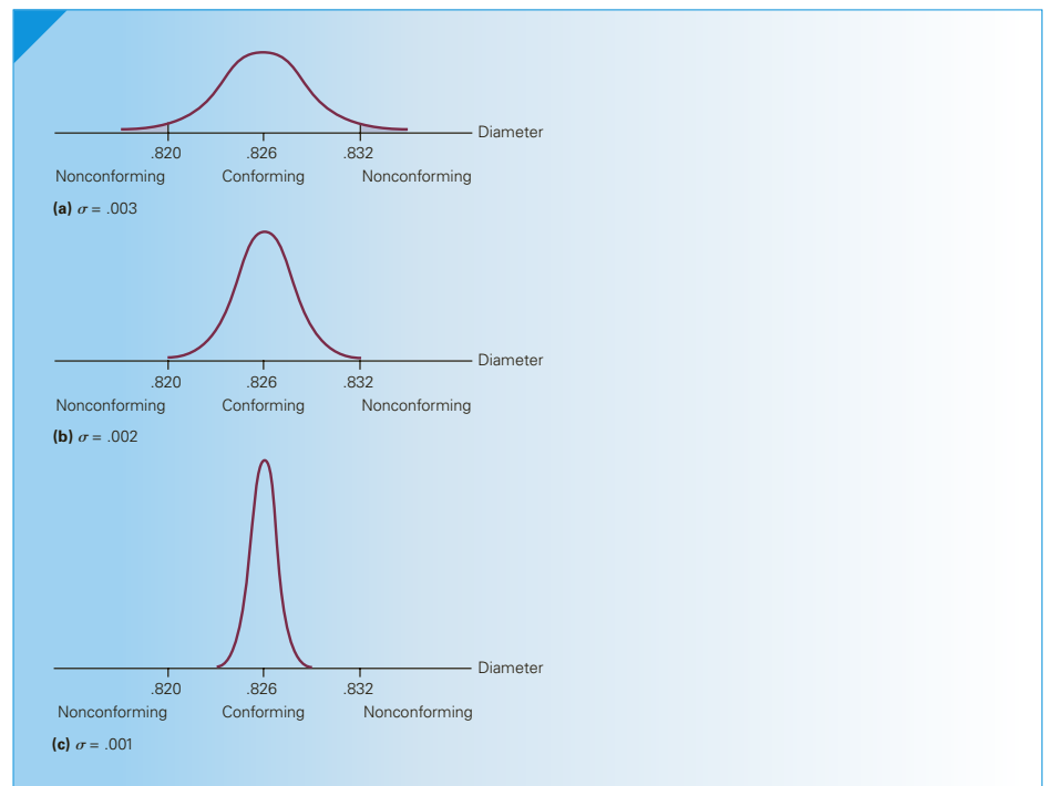
FIGURE 14.7 Proportion of Conforming and Nonconforming Piston Rings
